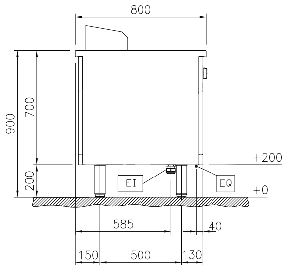
Lateral
